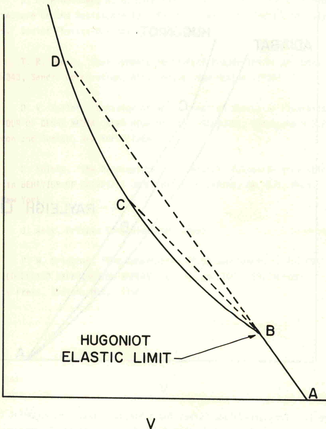
Figure 2. Hugoniot Curve for a Solid Showing a Cusp at the Elastic Limit. A single shock front is stable at stresses less than "B" or greater than "D". Intermediate shock amplitudes propagate as two wavefronts.
